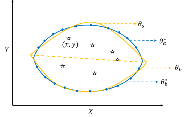
Fig. 2. Polynomial curve fitting.
