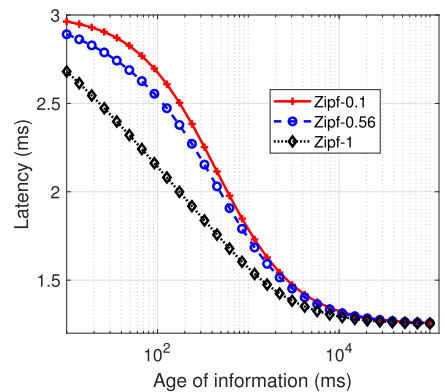
Fig. 11. Influence of content popularity (ReA scheme), R_{UL} = R_{DL} = 1000 /s, request arrival rate \Lambda = 200 /s.
