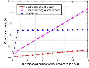
Fig. 9. Computation delay on \mathcal{U} and \mathcal{KS}_i in Register .
