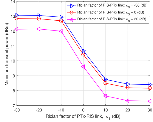
Fig. 7. Power versus Rician factors: Primary transmission requirement \Gamma_s = 20 dB, RIS transmission requirement \Gamma_c = 5 dB, number of reflecting elements N = 20 , spreading gain K = 100 .
