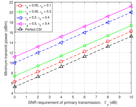
Fig. 8. Power versus uncertainty ratios, \epsilon_g and \epsilon_h : SIC factor \delta = 0.01 , number of reflecting elements N = 20 , RIS transmission requirement \Gamma_c = 5 dB, spreading gain K = 100 .
