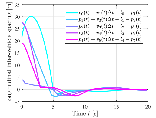
Fig. 7. The longitudinal inter-vehicle spacing of N = 5 platooning vehicles adopting the super-twisting SOSMDO-based controller.
