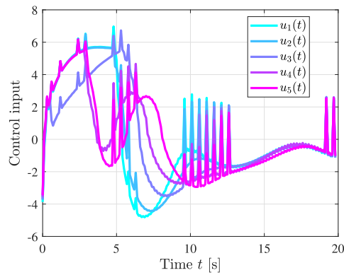
Fig. 5. The control inputs of N = 5 platooning vehicles adopting the super-twisting SOSM controller.
