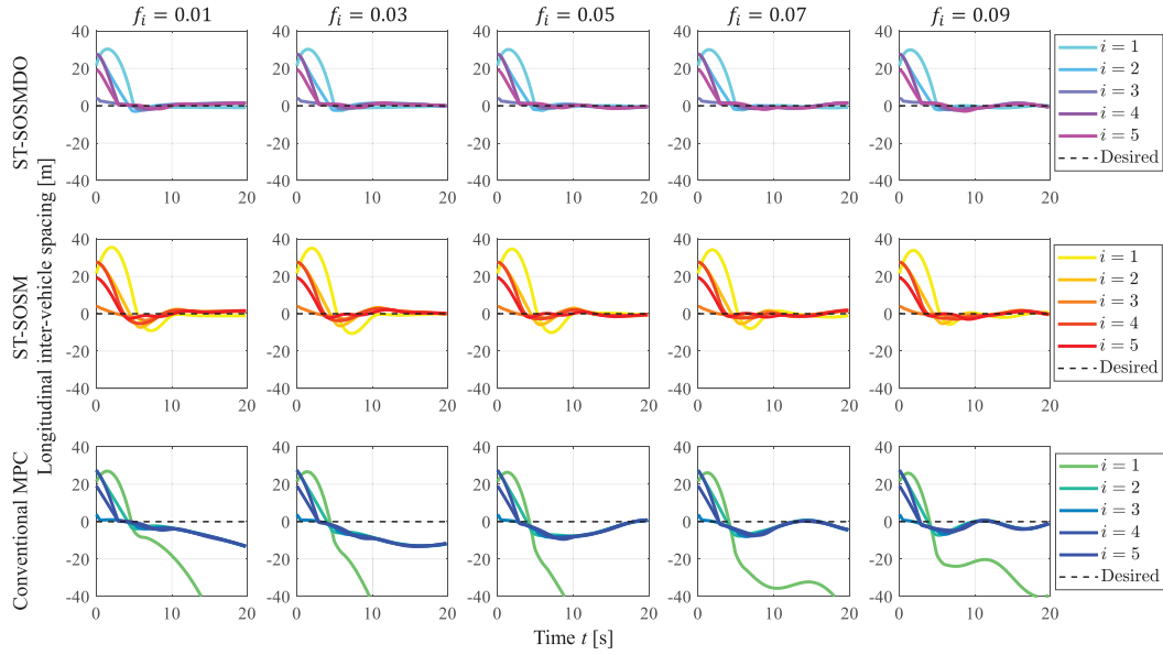
Fig. 13. The longitudinal inter-vehicle spacing of N = 5 platooning vehicles adopting different controllers under different disturbance frequencies.
