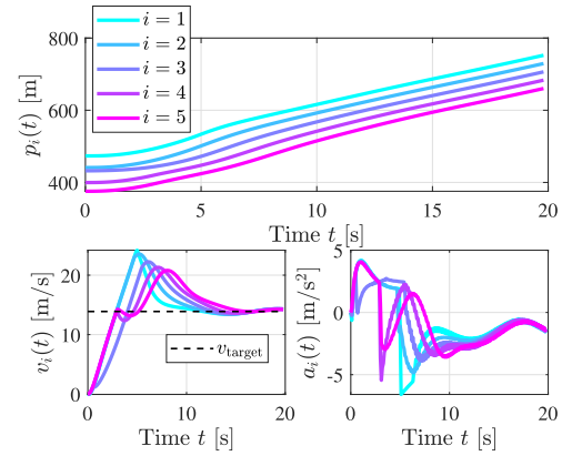
Fig. 6. The longitudinal positions, velocities, and accelerations of N = 5 platooning vehicles adopting the super-twisting SOSMDO-based controller.
