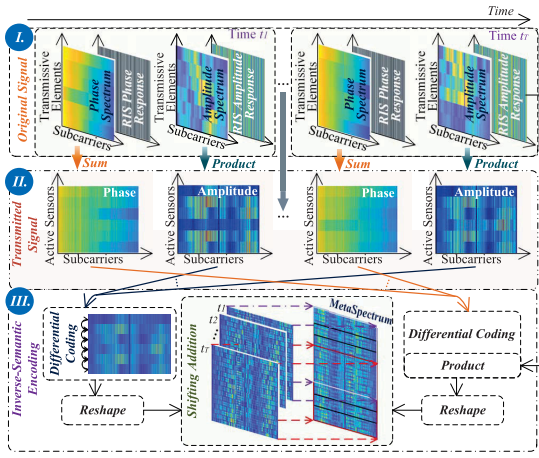
Fig. 3. The process of modulating the amplitude and phase spectrums through RIS, and then performing differential encoding and shifting addition.
