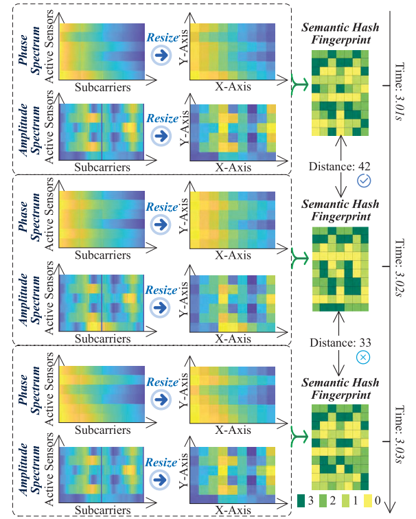
Fig. 4. The process of generating the resized matrices from the amplitude and phase spectrums, and then obtaining the semantic hash fingerprint.
