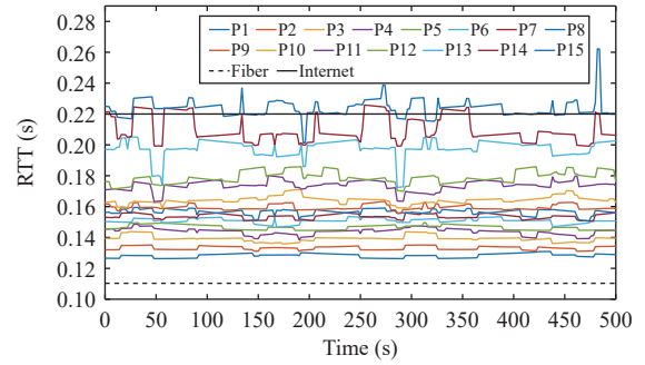
(a) RTT on 15 optimal paths from New York to Beijing in Phase 1
