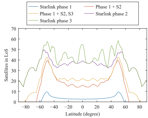
Fig. 8. Ground coverage features of Starlink.
