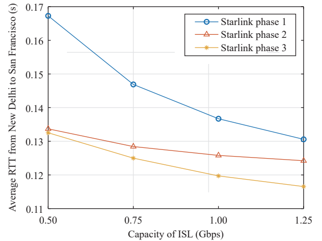
Fig. 11. Influence of link capacity on network performance.
