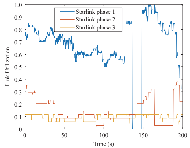
Fig. 14. Link utilization from New Delhi to San Francisco.
