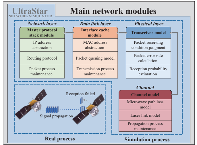
Fig. 5. The structure of UltraStar network module.
