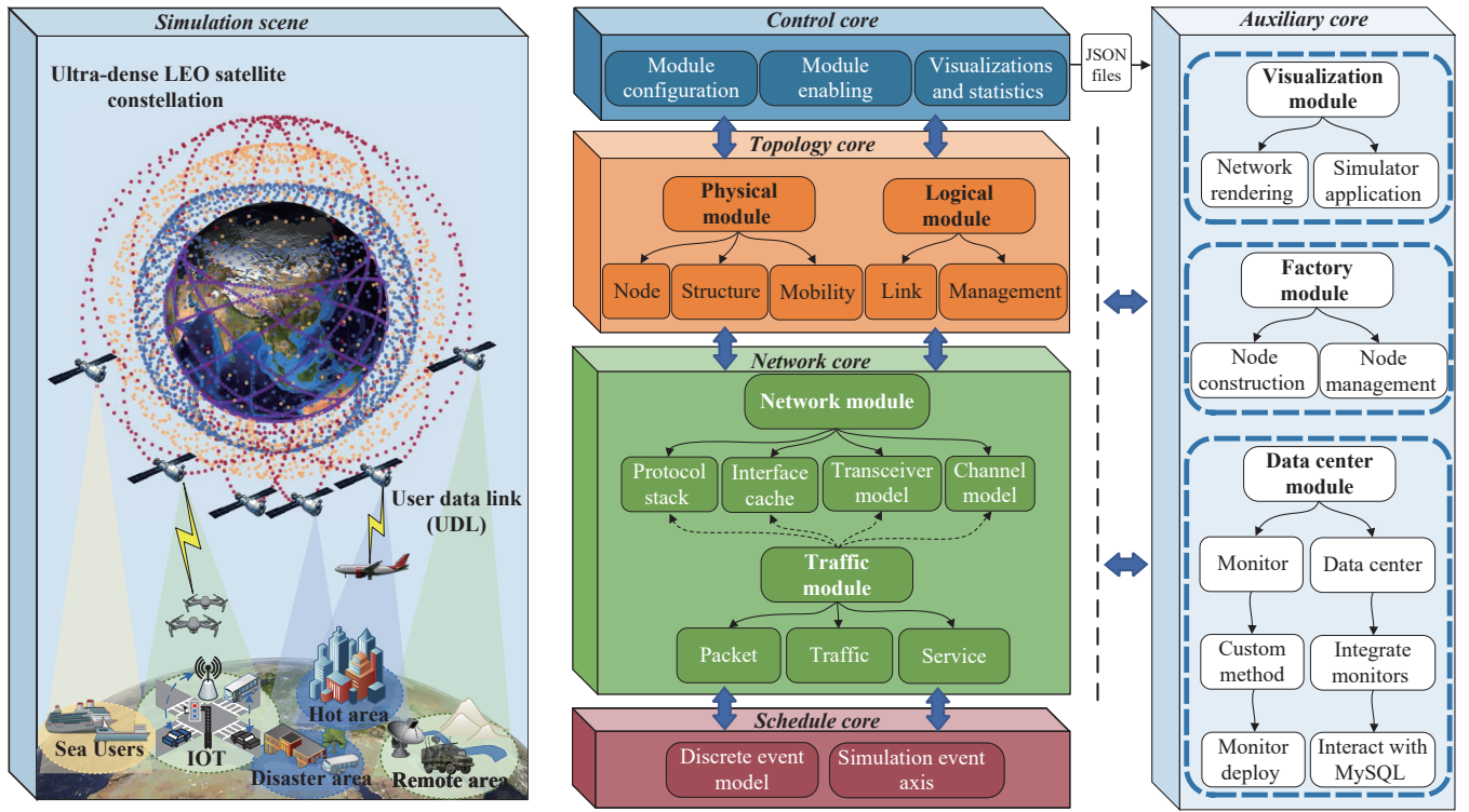
Fig. 1. The software architecture of UltraStar.
