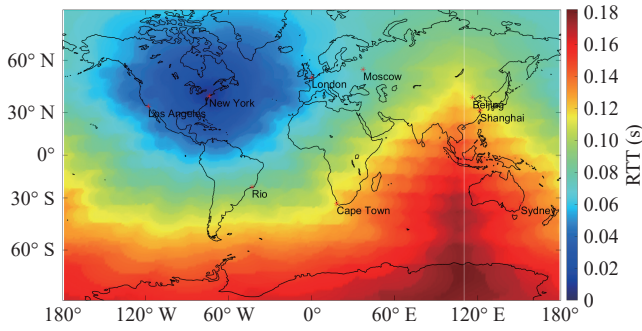
Fig. 9. Global RTT distribution from New York.
