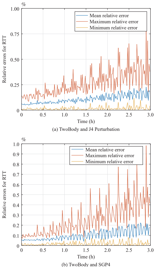
Fig. 15. Relative error of delay under different orbit prediction models.
