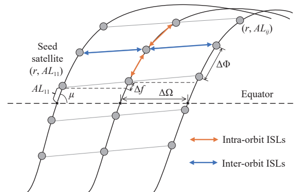
Fig. 4. Constellation topology and ISLs.
