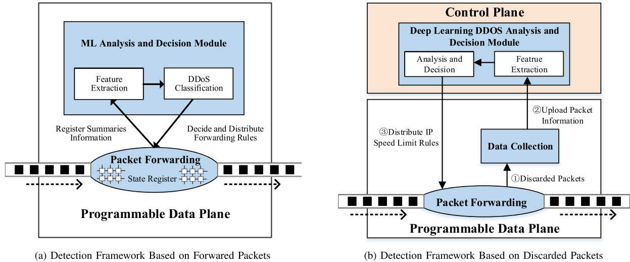
Fig. 6. Two Mechanisms about Defending DDoS Attacks with AI and PDP.
