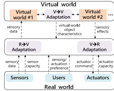
Fig. 3. The architecture of ISO/IEC 23005 (MPEG-V) standards [23]. R \rightarrow V adaptation means the conversion of sensory data from the real world (RW) to virtual world (VW) object characteristics. V \rightarrow R adaptation means the conversion of sensory effects from VW into actuator commands to RW. V \rightarrow V adaptation means the conversion of native representations of information in a VW to the standard format.
