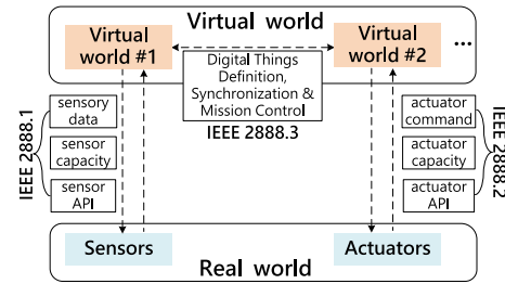
Fig. 4. The architecture of IEEE 2888 standards [24]. IEEE 2888.1, IEEE 2888.2, and IEEE 2888.3 specify the standards on sensor interface, actuator interface, and orchestration of digital synchronization, respectively.
