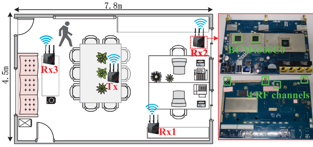
Fig. 8. Test scenario and hardware equipment.
