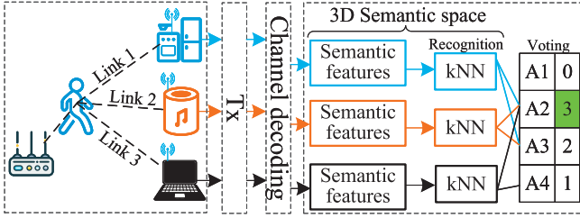
Fig. 7. Fusion of recognition results from multiple links.
