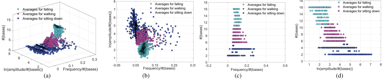
Fig. 6. Distribution of features averages in the 3D semantic space.
