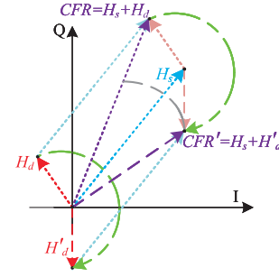
Fig. 2. Impact of the H_d phase on the overall CFR power.
