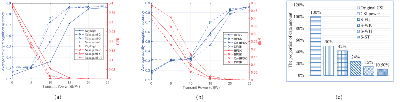
Fig. 10. Impact of wireless transmission on recognition accuracy and the data amount comparison before and after semantic encoding.
