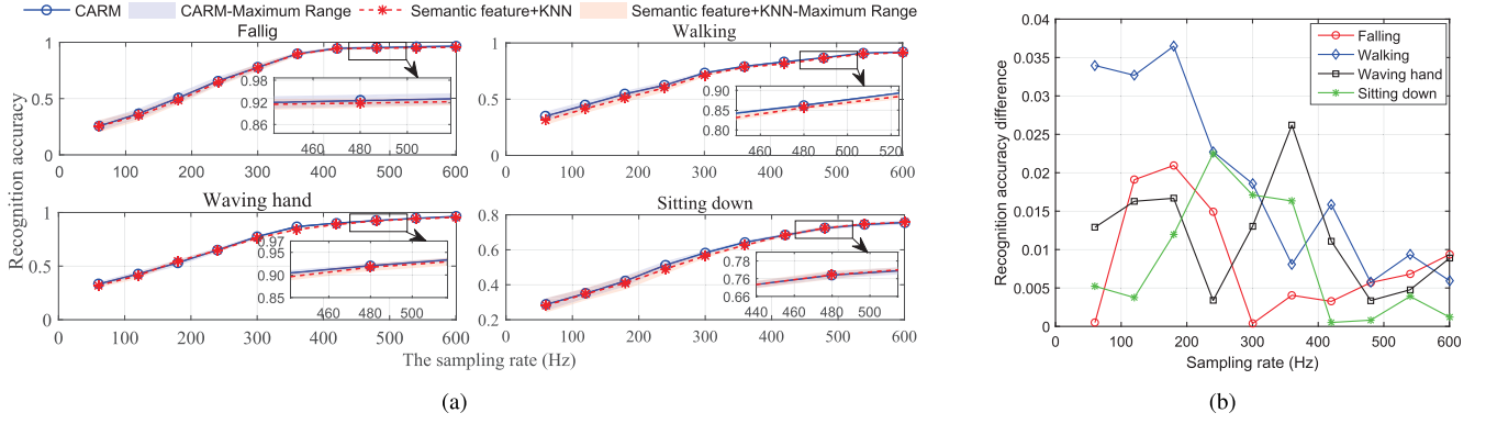
Fig. 9. Activity recognition accuracy in the 3D semantic space.
