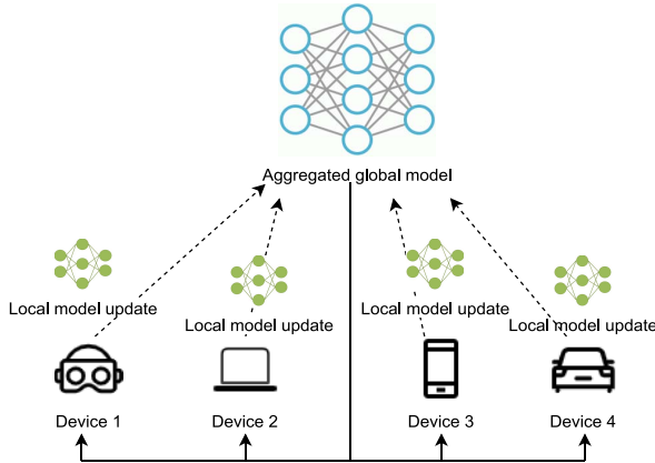
Fig. 12. Federated learning in edge networks.
