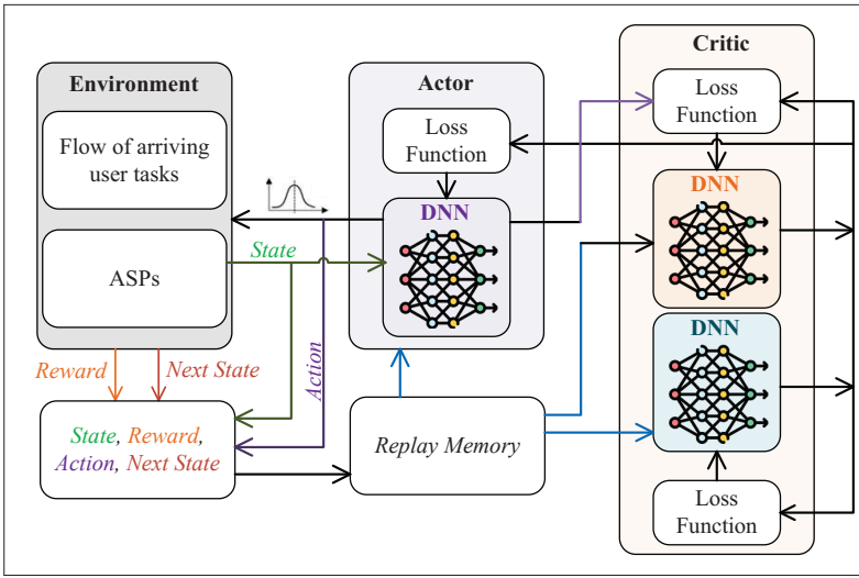
FIGURE 4. The structure of soft actor-critic DRL algorithm. The actor network is used for action selection and the critic networks are used for reward estimation.
