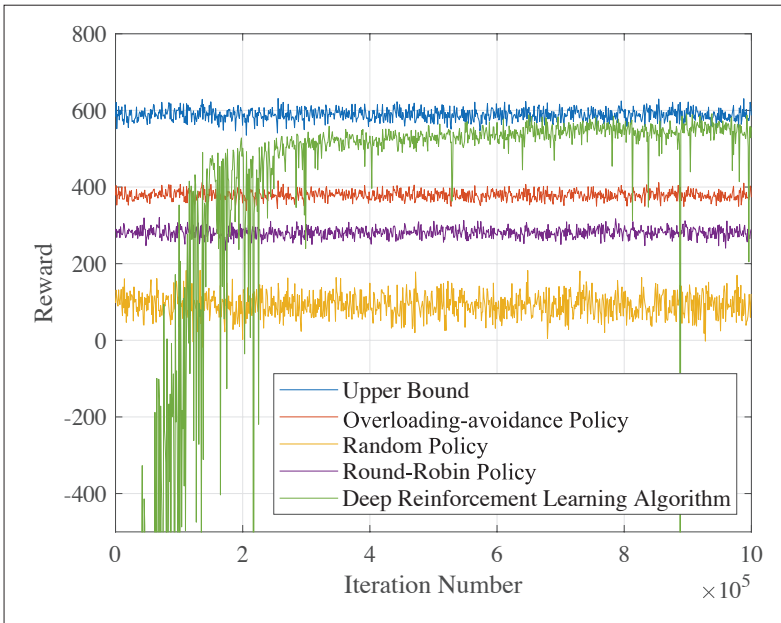
FIGURE 5. Reward values versus the number of iteration number in DRL. For performance comparison, we show the results of overloading-avoidance, random, round-robin policies, and their upper bound.
