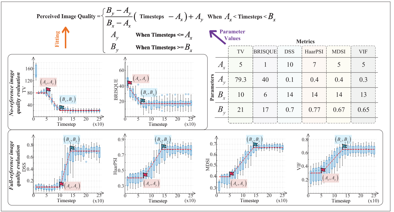
FIGURE 3. The relationship between the number of inference steps and various perceived image quality metrics, that is, TV, BRISQUE, DSS, HaarPSI, MDSI, and VIF. A general model of the perceived image quality metric that contains four parameters is presented.
