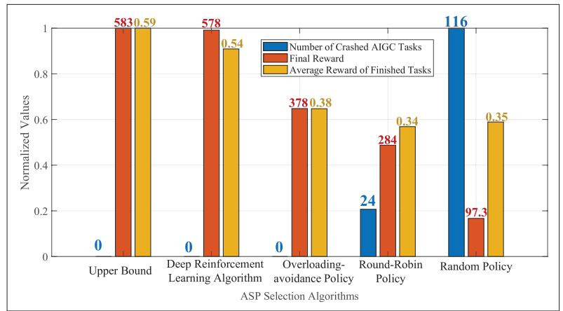
FIGURE 6. Comparison of episodic rewards, average rewards of finished tasks, and number of crashed tasks.
