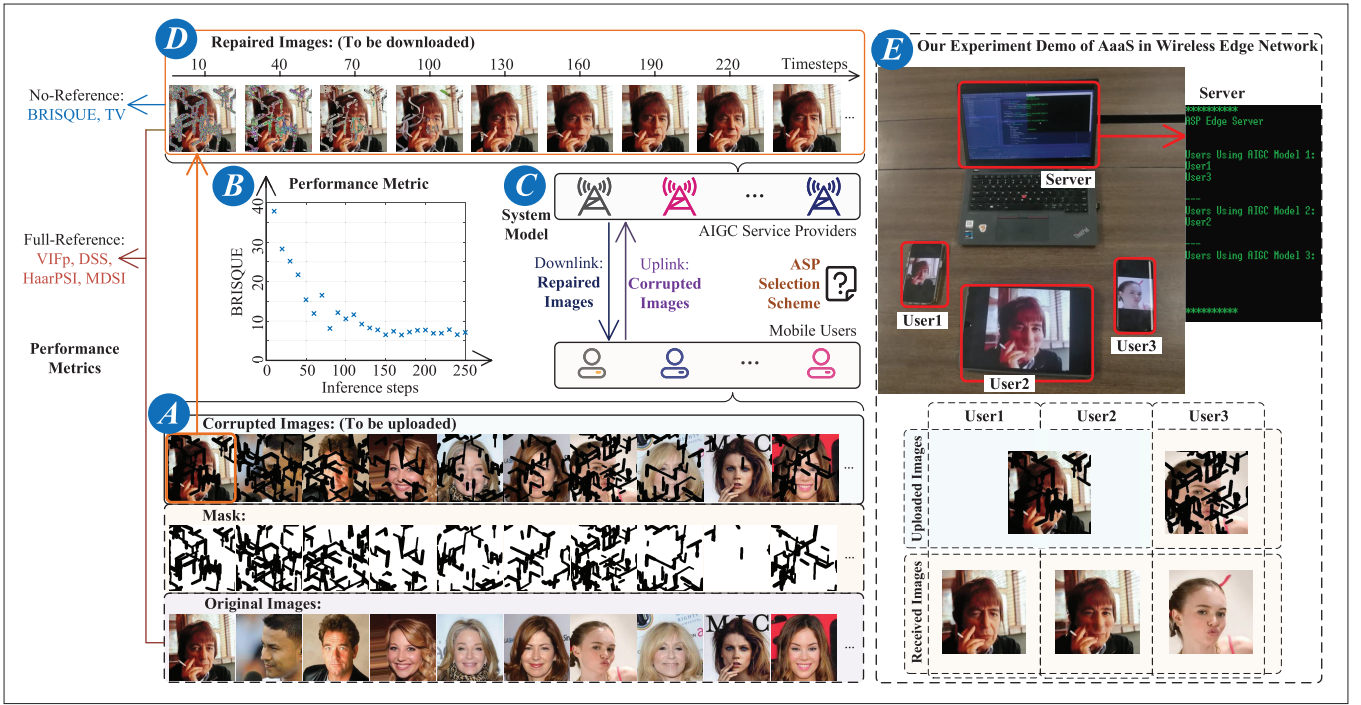
FIGURE 2. Example of an AaaS for repairing corrupted images. The corrupted images are shown in Part A, and the repaired images under different inference steps are shown in Part D. Part B shows how the performance metric, BRISQUE, varies over different inference steps. Part C shows the system model of ASP selection problem. A experiment demo is shown in Part E.
