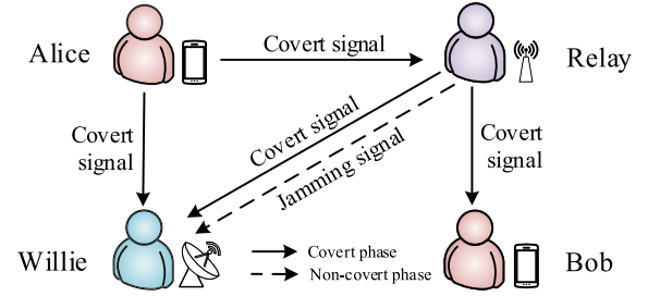
Fig. 10. Covert communications with the help of a relay with its dual roles, i.e., a cooperative jammer and an AF relay node. As the role of a cooperative jammer, the relay transmits the jamming signal in [132] while forwarding the received noise in [31] in the noncovert transmission phase. As the role of an AF relay, the transmitter Alice tries to communicate with Bob covertly in the presence of an adversary Willie in the covert transmission phase.
