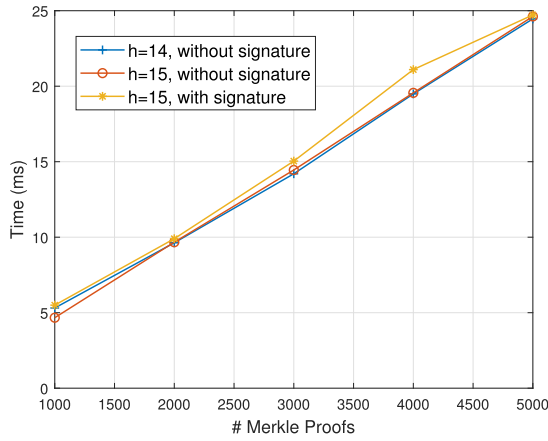
Fig. 8. Computation overhead of SGX-based pruning.
