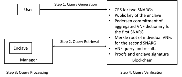
Fig. 5. Query workflow.
