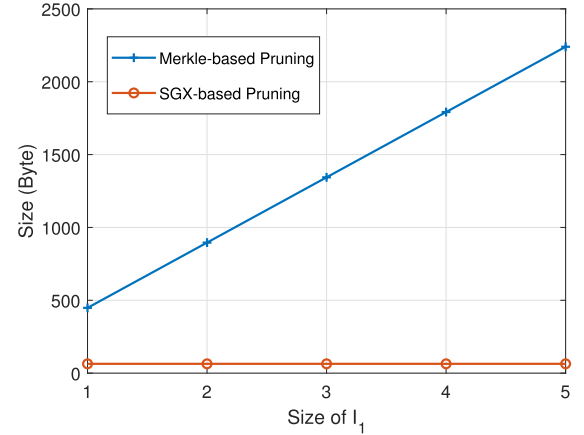
Fig. 7. Communication overhead.
