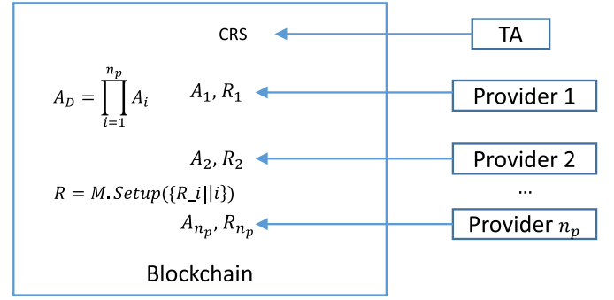
Fig. 3. Authenticator generation.
