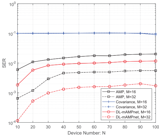
Fig. 11. SER performance versus device number N with different number of receiving antennas M .
