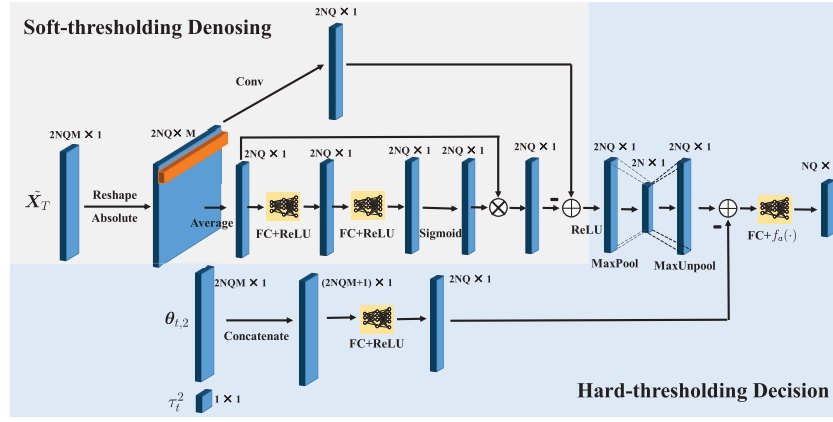
Fig. 5. Detailed architecture of the proposed refinement module.
