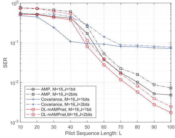
Fig. 10. SER performance versus pilot sequence length L with different lengths of transmitted messages J .
