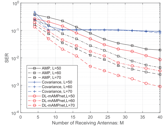
Fig. 9. SER performance versus number of receiving antennas M for J = 1 bit.
