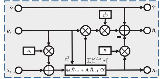
Fig. 4. Detailed structure of the t th AMP layer.
