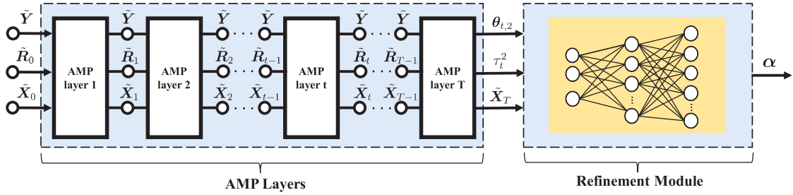
Fig. 3. Network architecture of the proposed DL-mAMPnet.
