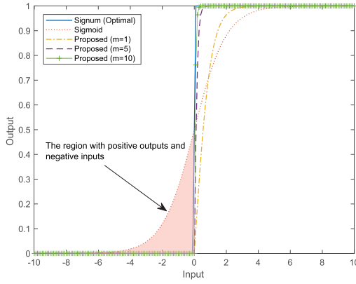
Fig. 7. The curves of the optimal signum, sigmoid, and hard-thresholding decision functions.
