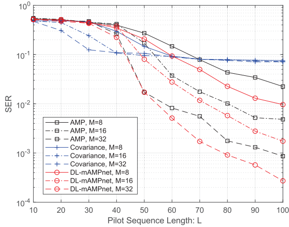
Fig. 8. SER performance versus pilot sequence length L for J = 1 bit.
