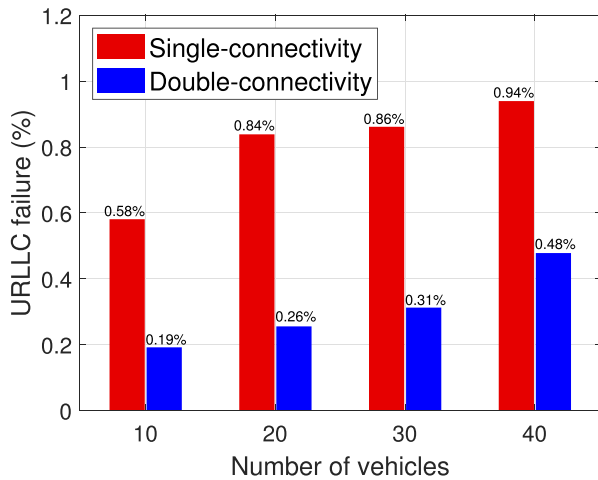
Fig. 6. URLLC failure percentage vs number of vehicles.
