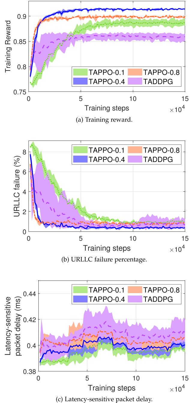
Fig. 4. Performance variation during training process.
