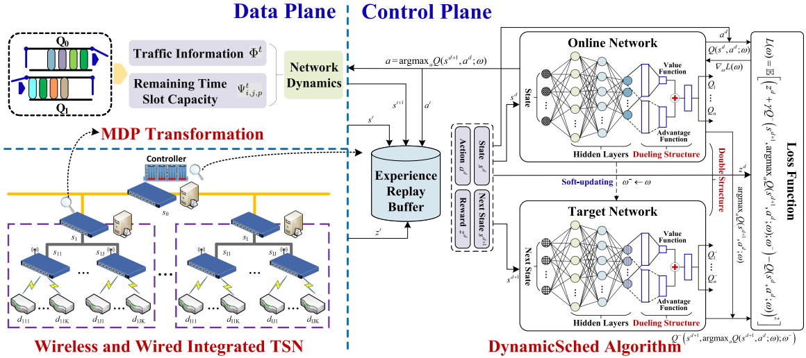
Fig. 3. Illustration of the proposed DynamicSched algorithm.
