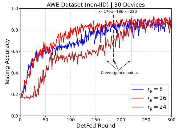
Fig. 6. Testing accuracy of DetFed with respect to different factory aggregation frequencies.
