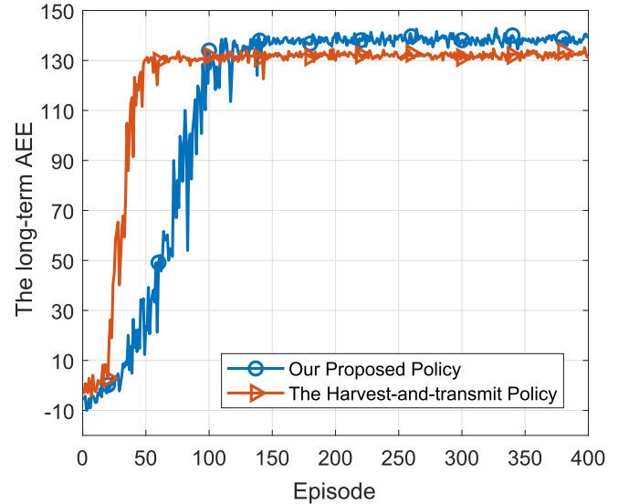
Fig. 6. The long-term AEE achieved by different policies.
