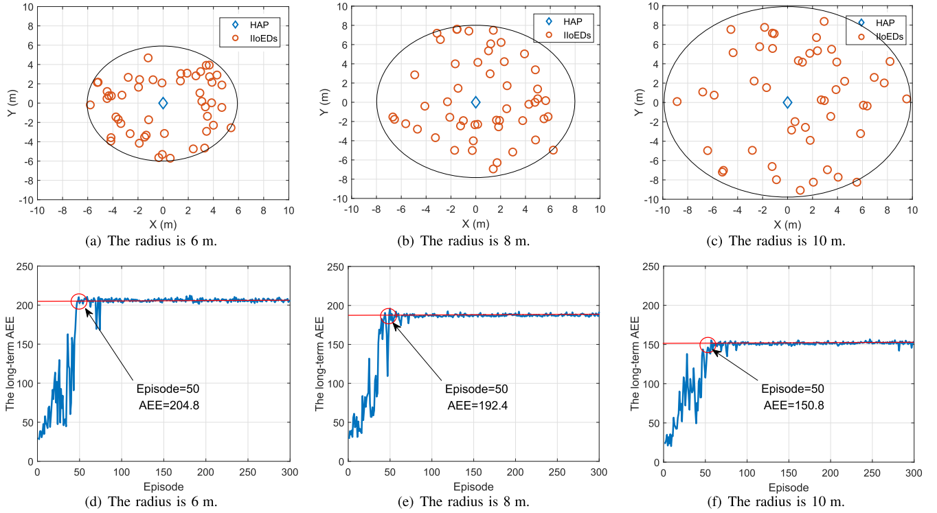
Fig. 8. The impact of distance between HAP and IIoEDs on the system long-term AEE.
