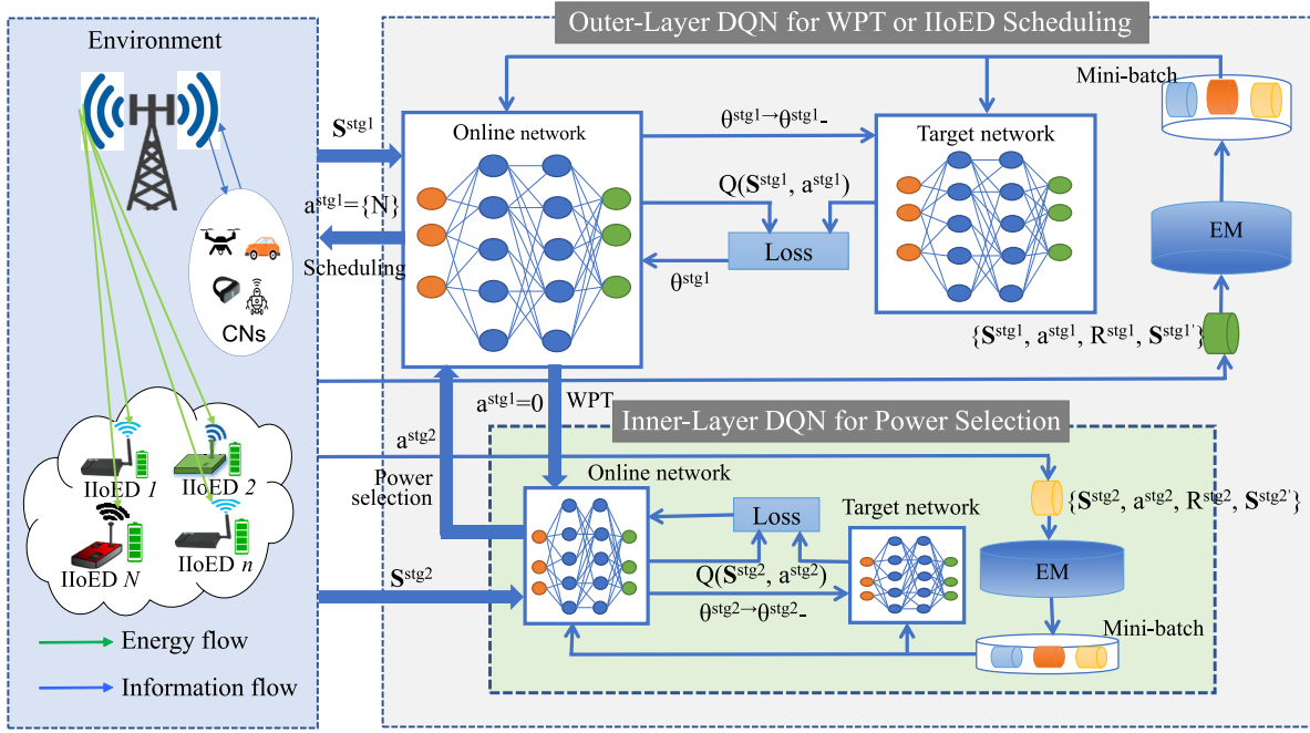
Fig. 4. Illustration of the framework of our proposed DLDQN algorithm.
