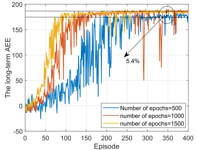
Fig. 11. The long-term AEE versus the number of epochs.
