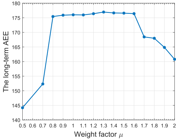
Fig. 12. The long-term AEE versus the weight factor in reward function.
