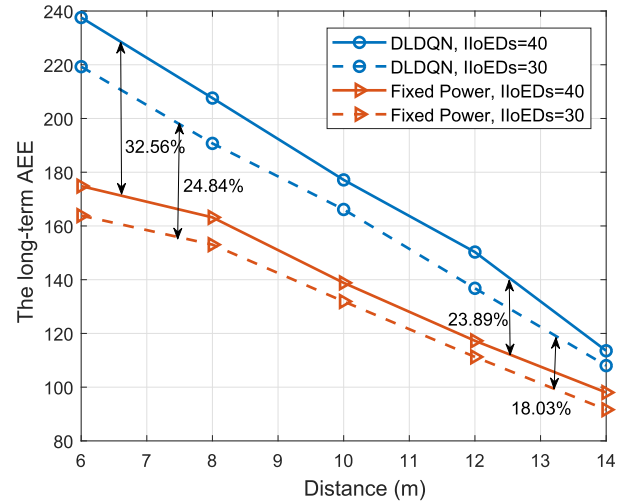
Fig. 9. The system long-term AEE versus the distance between HAP and IIoEDs.
