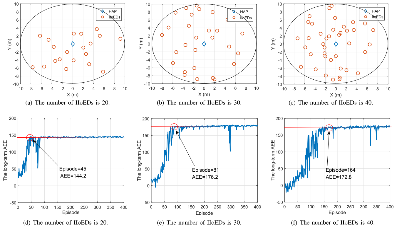
Fig. 10. The impact of the number of IIoEDs on the long-term AEE.
