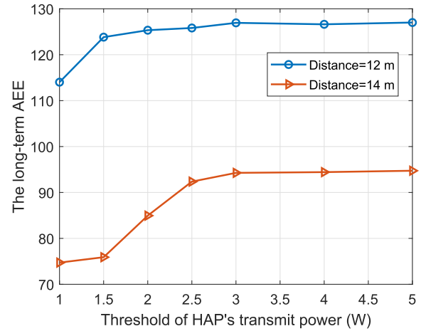
Fig. 15. The long-term AEE versus the threshold of HAP's transmit power.
