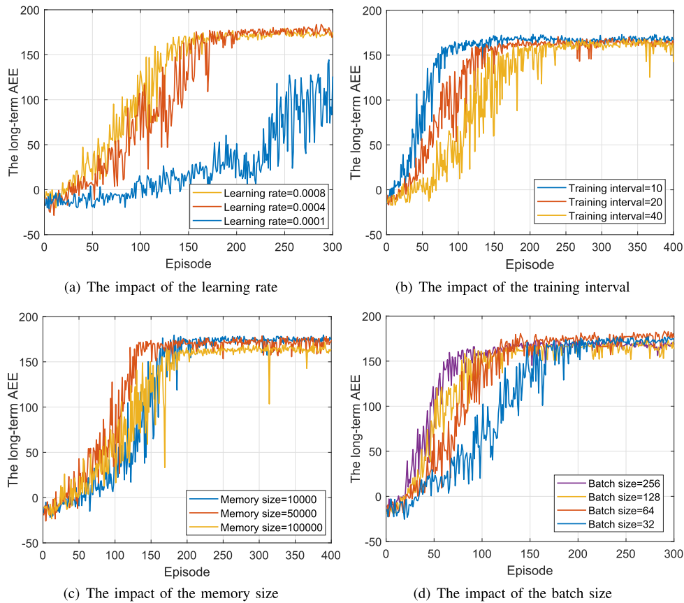
Fig. 7. The convergence performance of our proposed DLDQN algorithm with different network parameters.
