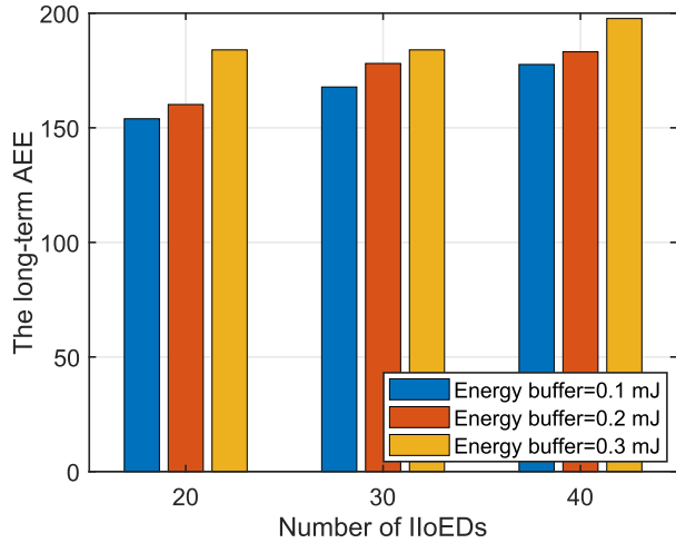
Fig. 13. The long-term AEE versus the energy buffer capacity.
