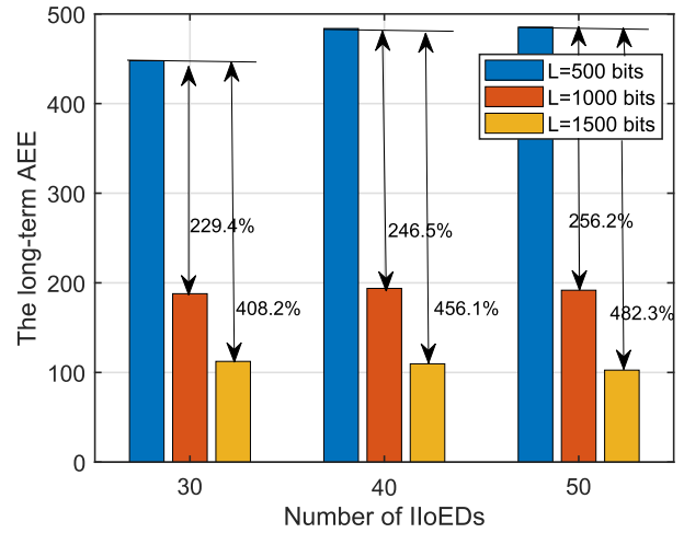
Fig. 14. The long-term AEE versus the update packet length.
