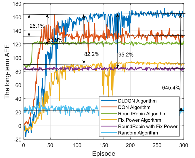
Fig. 5. The long-term AEE achieved by different algorithms.
