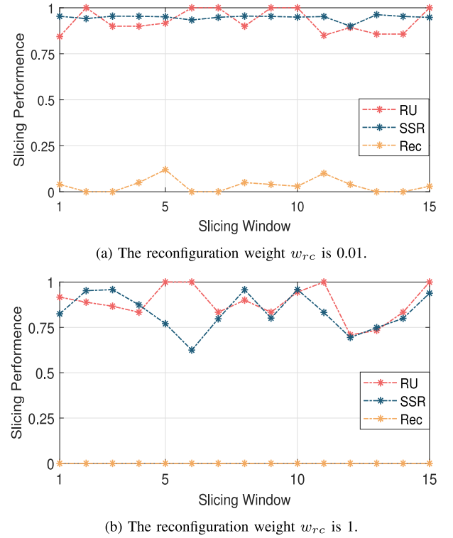
Fig. 10. Slicing performance in the different weight of the reconfiguration.
