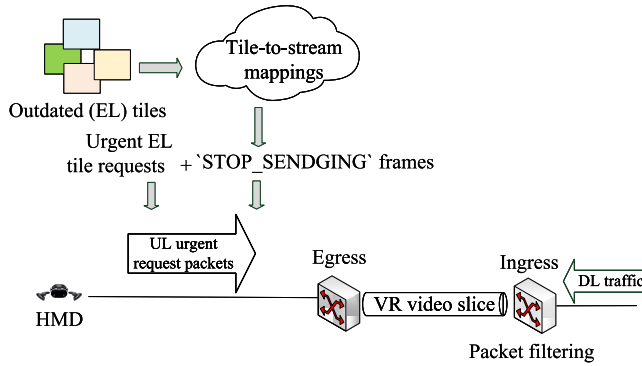
Fig. 8. The workflow of video packet filtering.
