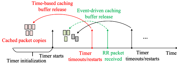
Fig. 10. The workflow of event-driven and time-based caching buffer releases.
