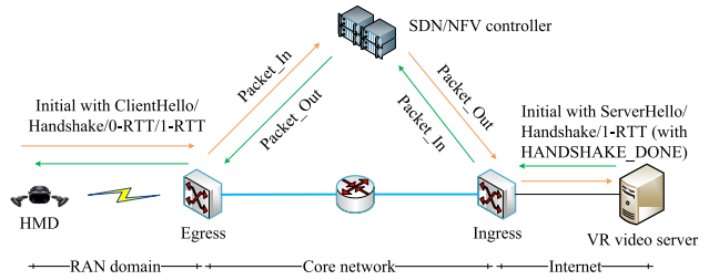
Fig. 4. SDN/NFV-based E2E QUIC connection establishment.
