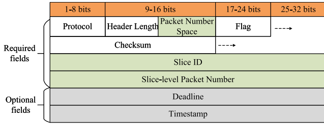
Fig. 5. The slice-level packet header format.
