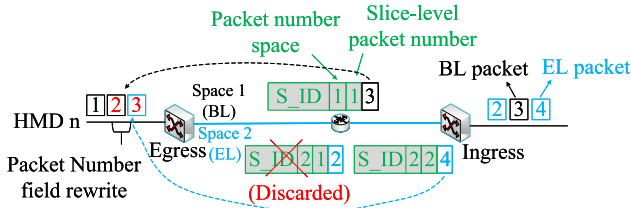
Fig. 6. Video packet transmission over a VR video slice.
