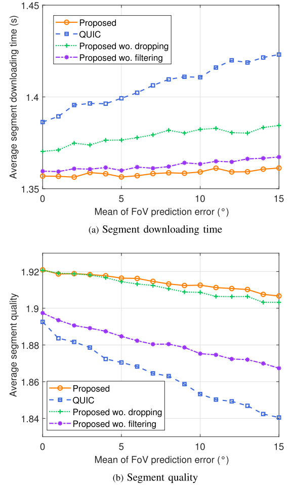
Fig. 15. Average segment downloading time and quality vs. FoV prediction error.
