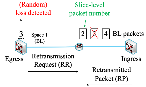
(a) BL packet loss detection and retransmission.
