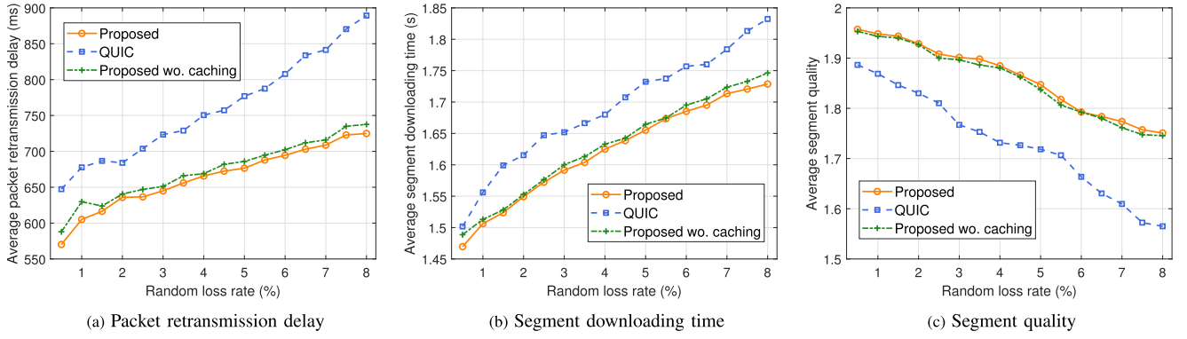
Fig. 14. Average packet retransmission delay, segment downloading time, and segment quality vs. random packet loss rate.
