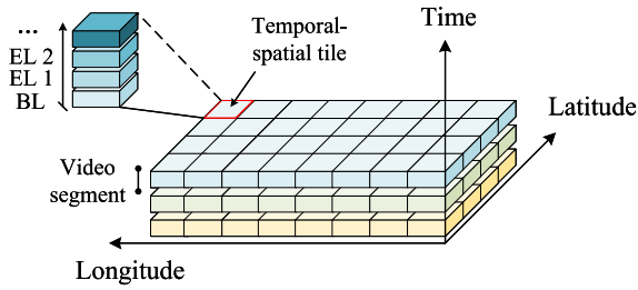
Fig. 2. Tile-based VR video encoding.
