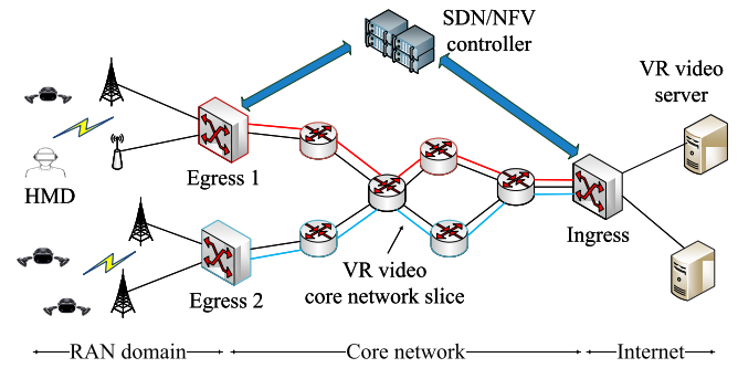
Fig. 1. The SDN/NFV-based E2E transmission network scenario.
