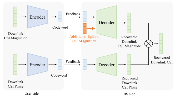
Fig. 16. Uplink CSI aided downlink CSI feedback in massive MIMO FDD systems.
