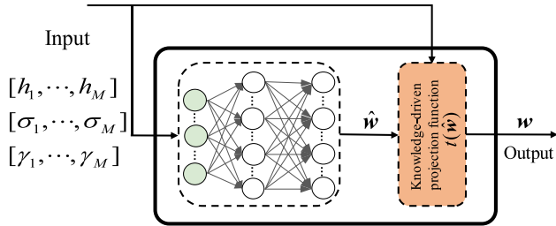
Fig. 8. A knowledge-driven projection function for multicast beamforming.
